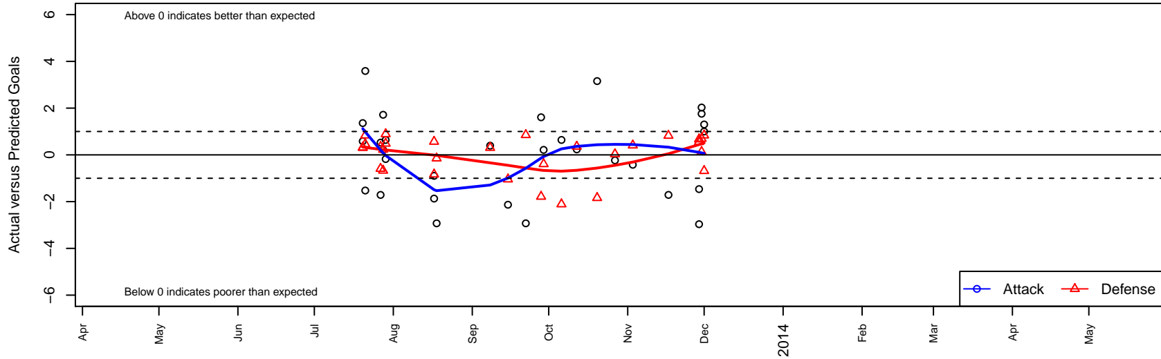
FC Golden State Diamond B96 Dots are actual minus expected GF (blue circles) and GA (red triangles). Blue line is smoothed change in attack strength. Red is smoothed change in defense strength.
